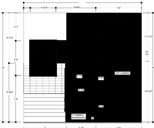
S3 SECTION 3 201 1/2" = 1'-0"
